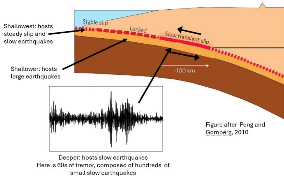
The common distribution of slow and fast earthquakes in a subduction zone.
