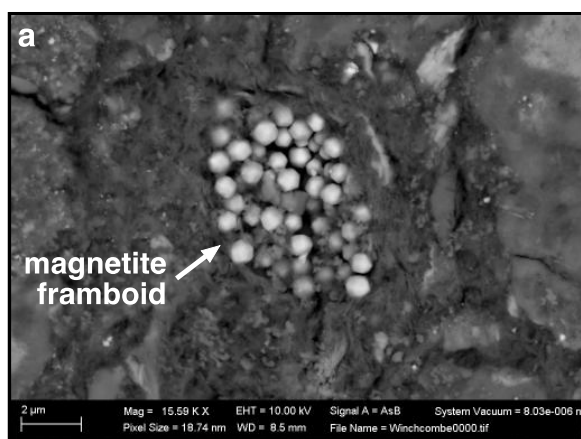
Figure 1: magnetite framboids in the Winchcombe meteorite (modified by Bryson et
