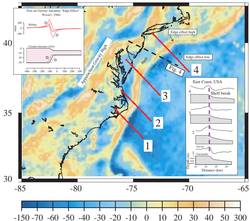
Figure 1. The free-air gravity anomaly field of the east coast (U.S.) based on DNAG data.
