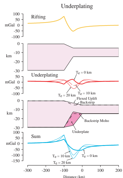
Figure 3. The gravity anomaly associated with magmatic underplating and its influence on the anomaly due to rifting based on a density of the underplated material of 2900 kg/m 3 (other densities as in Figure 2) and elastic thickness values of 0, 10, and 20 km.
