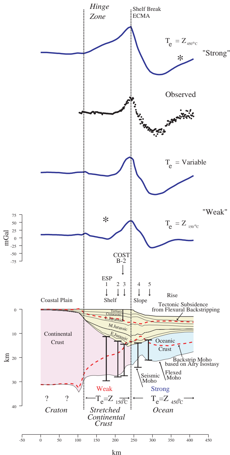
Figure 4. Combined back-stripping and gravity modeling of a seismically constrained profile of the Baltimore Canyon Trough (see Figure 1 for profile location). The black dots show the observed free-air anomaly based on shipboard measurements. The blue profiles show the calculated anomalies obtained by combining the rifting and sedimentation anomalies. Three cases of margin strength have been considered: one (upper profile) that corresponds to oceanic lithosphere; one (lower profile) that corresponds to rifted continental lithosphere; and a combination of both cases.
