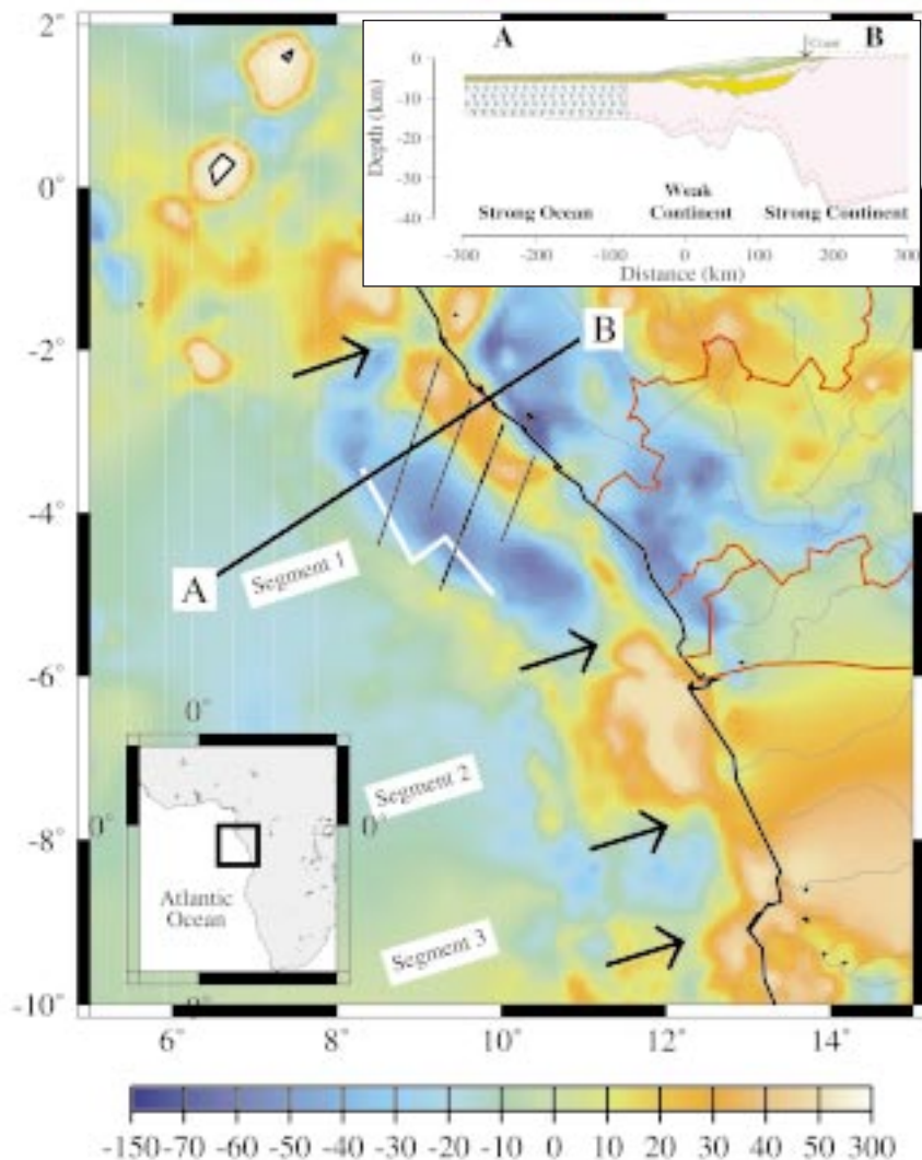
Figure 5. The gravity anomaly field (Bouguer onshore, free-air offshore) of the West Africa margin based on GETECH data. Upper right inset shows the interpreted crustal structure along Profile AB of the Gabon margin, based on a combined back-stripping and gravity modeling approach.
