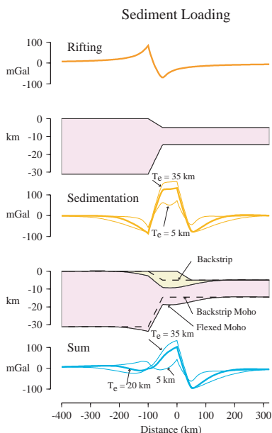
Figure 2. The gravity anomaly associated with sediment loading and its influence on the anomaly due to rifting based on an assumed density of the water, crust, and mantle of 1030, 2400, and 3330 kg/m 3 , respectively, and elastic thickness values of 5, 20, and 35 km.
