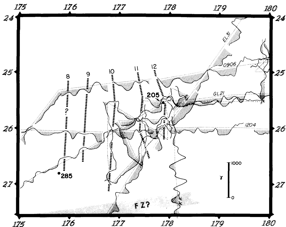
Fig. 2. Detailed map of the north-south magnetic lineations in the east-central part of the South Fiji basin. Magnetic anomaly "lows" are shaded.
