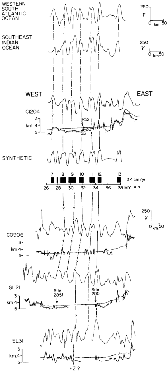
Fig. 3. Comparison of projected magnetic anomaly profiles with a computed profile and profiles from major ocean basins. The South Fiji basin magnetics and line drawings of seismic reflection profiles have been projected normal to the lineation direction. The computed profile assumes a depth to upper surface of the block model of 4.9 km, a layer thickness of 0.5 km and a uniform magnetization contrast of 0.005 \text{ emu/cm}^3 . The profiles from other ocean basins have been phase-shifted by 10^\circ and plotted at horizontal and vertical scales to match observed anomalies in the South Fiji basin. The dagger adjacent to 285 indicates that the position of this site has been projected on to the GL21 profile, whereas it really lies about 25 km south of this track (Fig. 2).
