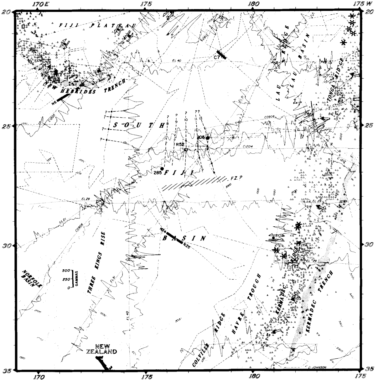
Fig. 1. Marine magnetic anomalies along ship tracks in the South Fiji marginal basin. Dotted lines are ship tracks of Lamont-Doherty Geological Observatory and the Deep-Sea Drilling Project and dashed lines are tracks from other sources. Bathymetry [20] is shown at 100-fm contour intervals. Historically active volcanoes are indicated by asterisks and earthquake epicenters with focal depths less than 100 km by open triangles. Hollow arrows indicate focal mechanism solutions of selected shallow earthquakes [21]. Solid circles indicate DSDP sites [15,17], solid bars indicate seismic refraction profiles [8], and the open circle is sonobuoy refraction station R52.
