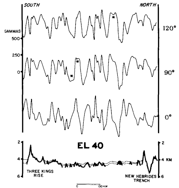
Fig. 4. EL40 magnetic anomaly profile (Fig. 1) phase-shifted by 120^\circ , 90^\circ , and 0^\circ (top three profiles). Although most anomaly shapes passed through symmetry after 90^\circ to 120^\circ of phase-shifting, asterisks denote the prominent magnetic anomalies which have been brought to symmetry. The bottom profile is a line drawing of the corresponding EL40 seismic reflection profile.
