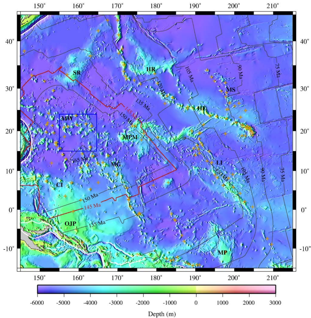
Fig. 1. Bathymetric map of the Jurassic and Cretaceous age Pacific Ocean based on the GEBCO 1 \times 1 minute grid and seafloor age data from (Müller et al., 2008) showing selected features referred to in the text. The thick red contour marks the boundary between Jurassic and Cretaceous seafloor. Yellow crosses show the locations of dated samples (Clouard and Bonneville, 2005; Koppers and Staudigel, 2005) used to determine the lithosphere age at the time of loading. Plate boundaries are marked with a heavy white line. The blue box delineates the area used to calculate the admittance in Fig. 2. Bathymetric features: CI, Caroline Islands; HE, Hawaiian-Emperor Seamount Chain; HR, Hess Rise; LI, Line Island Chain; MG, Marshall Islands and Gilbert Ridge; MP, Manihiki Plateau; MPM, Mid-Pacific Mountains; MS, Musician Seamounts; OJP, Ontong-Java Plateau; SR, Shatsky Rise; MW, Marcus-Wake Guyots.
